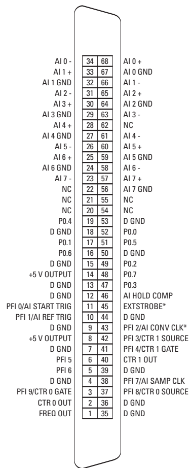
Figure 3. I/O Connector
