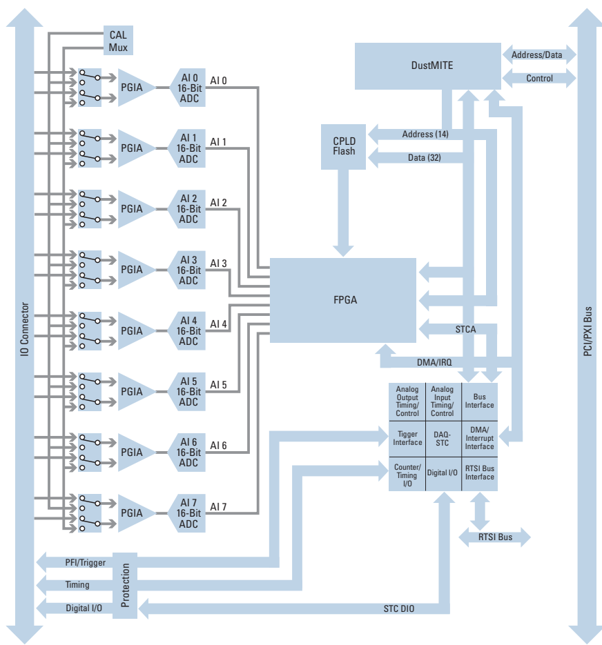
Figure 2. Block Diagram
